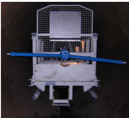
Paint-Sandblast trolley
